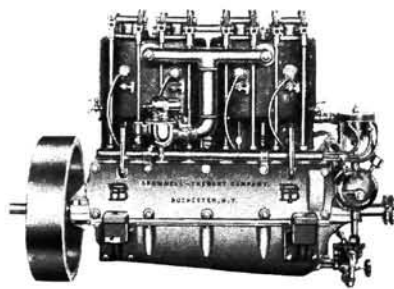
4 Cylinder. 30-35 H. P. B-T Motor.
