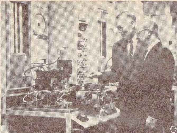
Loris H. Conrad (left), manufacturing manager, and Philip B. Zeigler, general manager of Rochester Products Division, General Motors Corporation, examine new computer-controlled carburetor test stand.
