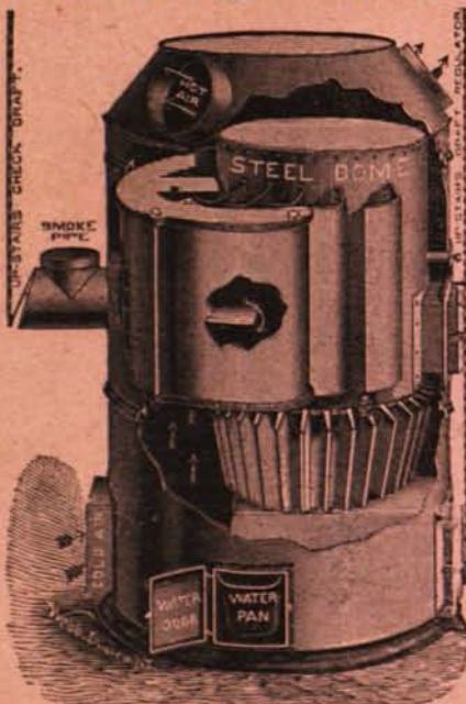
Steel dome and radiator, cast iron flanges on dome and fire-pot.
