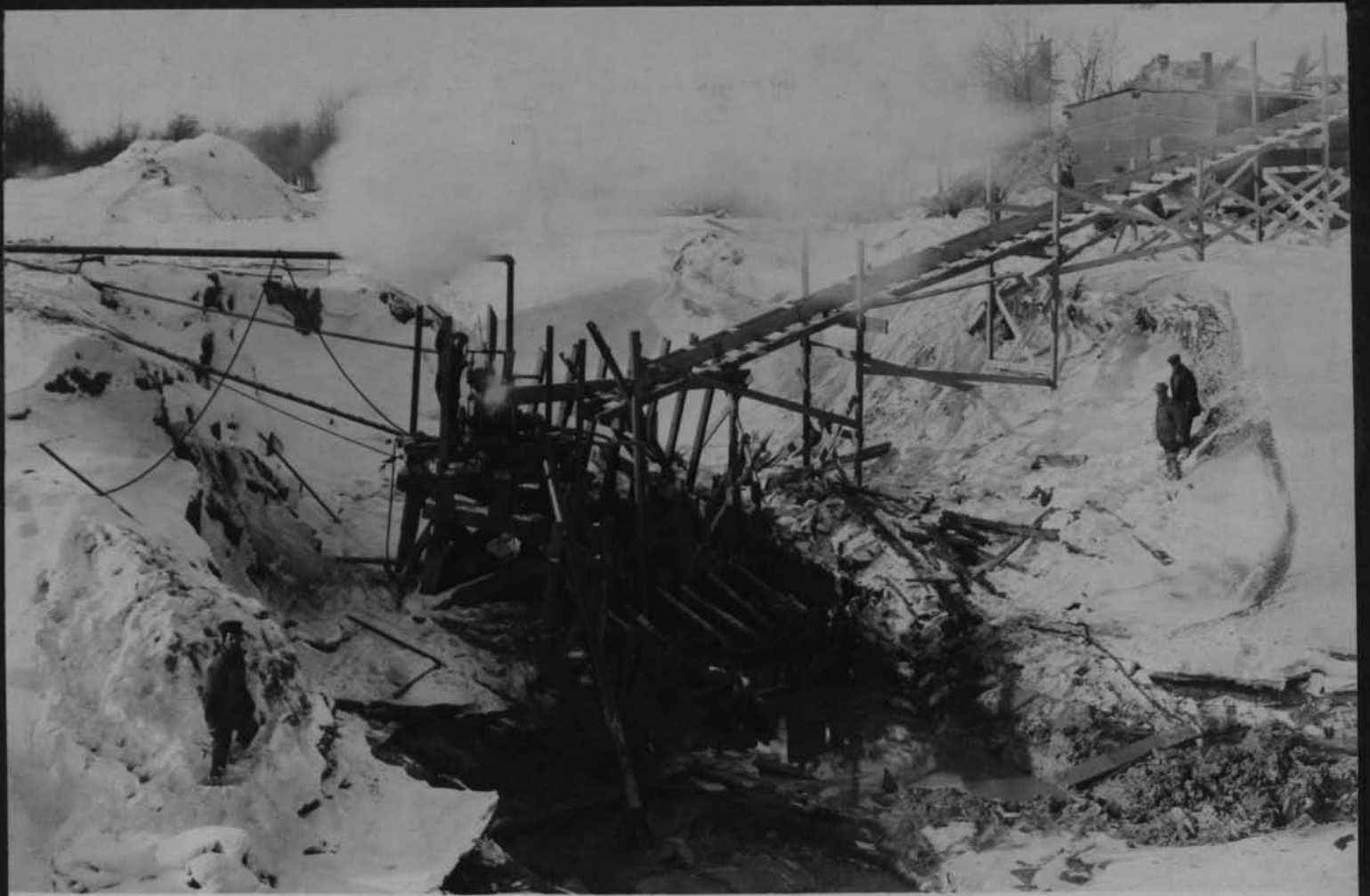
11584 Excavation for south abutment for foot bridge West side of Genesee Cont 59 Dec 18 1917
