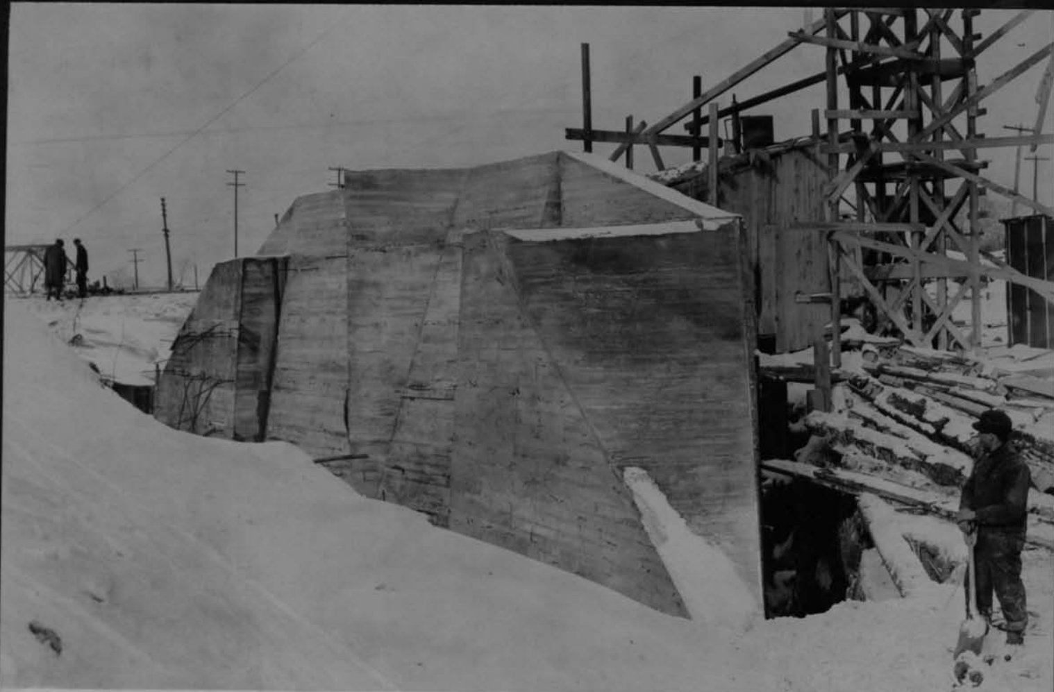
11634 South abutment for Penna R R crossing South Park Looking west Cont 59 Jan 25 1918
