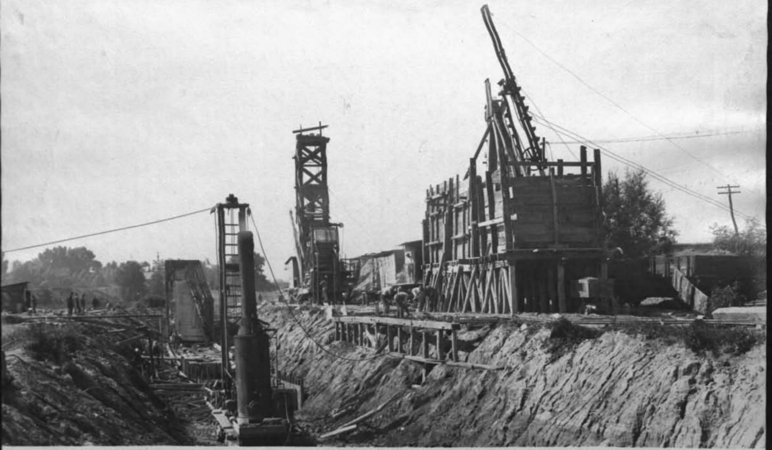
11447 River wall near Erie R R bridge Cont 59 Sept 13 1917
