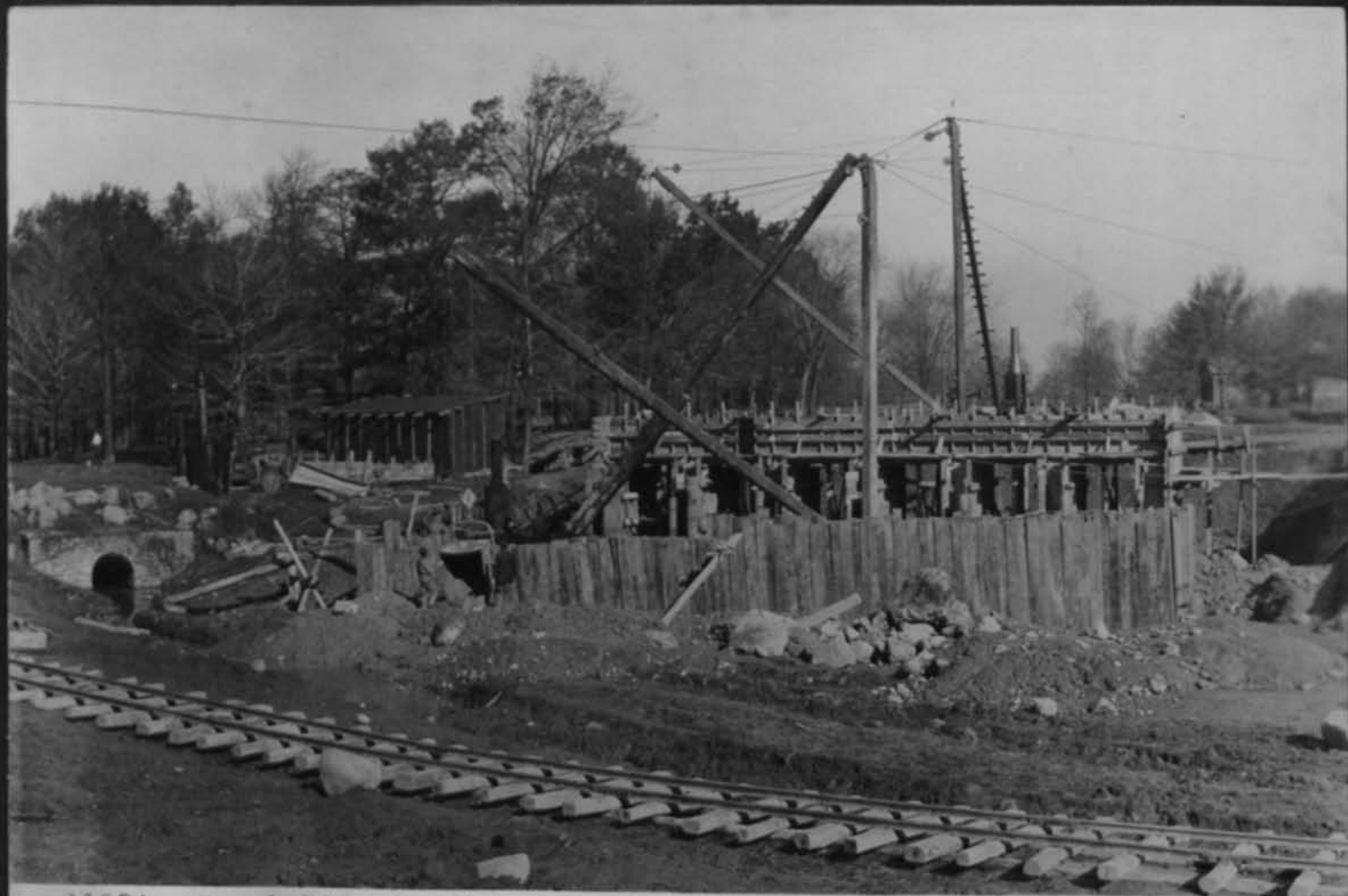
11534 North Pier for Main Drive Bridge Looking north Cont 59 Nov 5 1917
