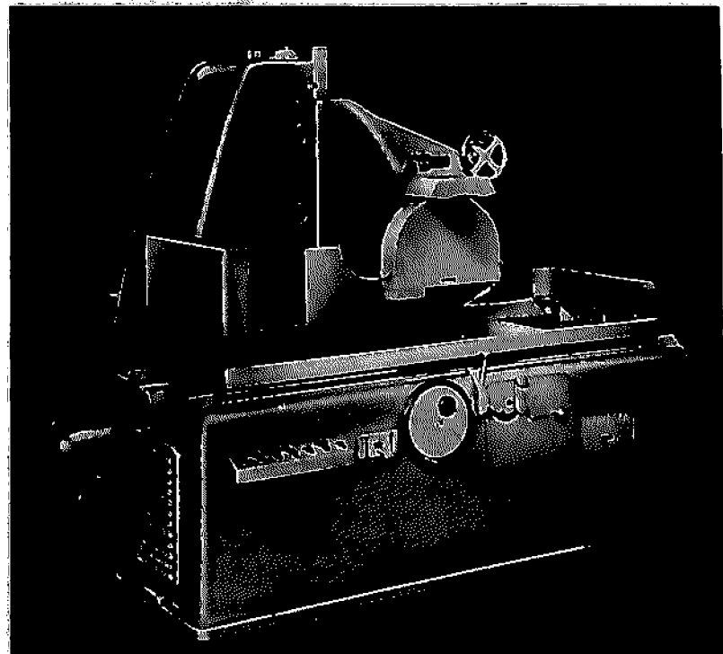
TYPE C—24" x 16" x 48" CAPACITY — THOMPSON HYDRAULIC SURFACE GRINDER
