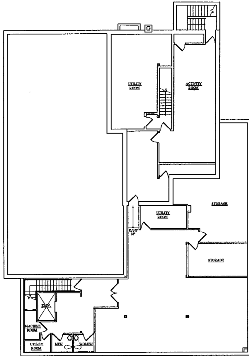
1 EXISTING FOUNDATION/ LOWER LEVEL PLAN 1/8"=1'-0"
