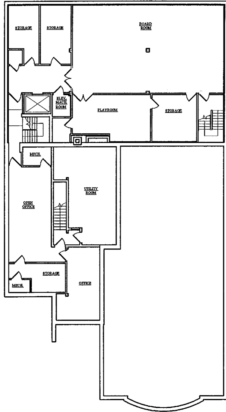
1 EXISTING FOUNDATION/LOWER LEVEL PLAN 1/8"=1'-0"
